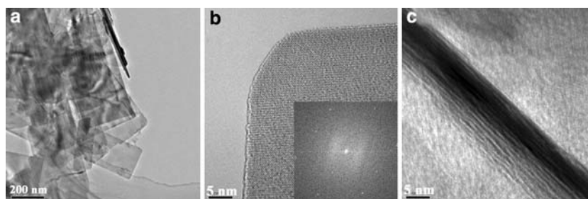
Figure 3. HRTEM photographs of products derived from hydrothermal reaction at 210 °C.
